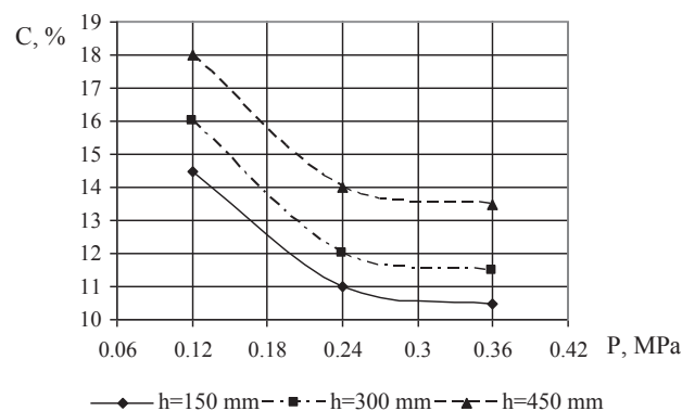
Fig. 5. Dependence of syrup concentration C in a mixed solution on the water supply pressure P at a blend syrup supply pressure of 150–450 mm and the annular clearance in the receiving chamber of 2.7 mm. The injector nozzle diameter is 8 mm, the distance between nozzles is 24 mm
