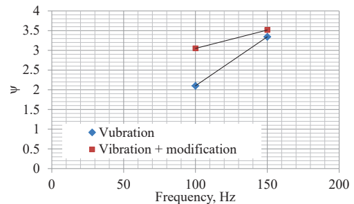
Fig. 5. \psi=\psi(f) dependence
