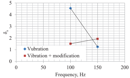
Fig. 4. \delta_s=\delta_s(f) dependence
