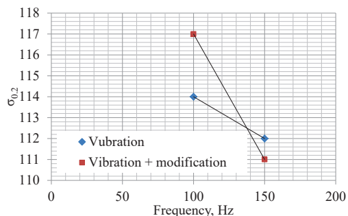
Fig. 2. \sigma_{0.2}=\sigma_{0.2}(f) dependence
