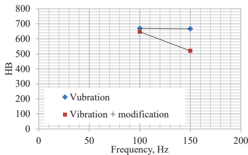
Fig. 1. HB=HB(f) dependence
