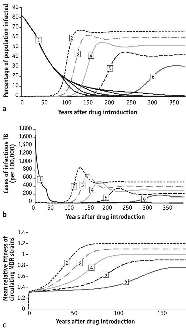
Figure 2. Sensitivity of long-term projections of MDRTB epidemics to the relative fitness of MDR strains
