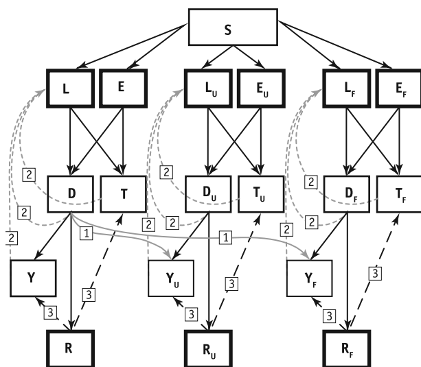
Figure 1. Multistrain tuberculosis model structure
