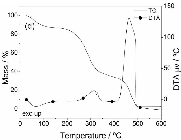
Figure 1 (continuation). TG-DTA curves for native (a) and modified corn starch with standard KMnO 4 at 0.01 mol L -1 (b); 0.02 mol L -1 (c) and 0.05 mol L -1 (d)
