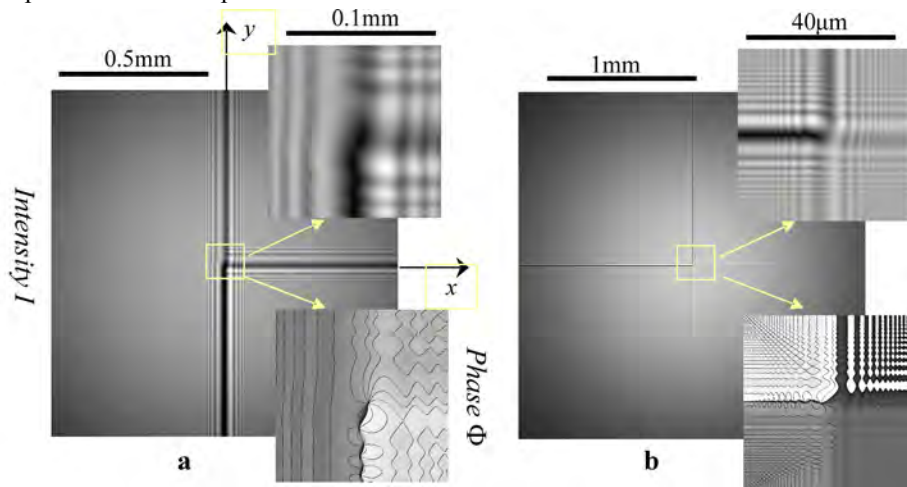
Fig. 8. Intensity and phase distributions in the beams with the \pi -cut: the pass-by with (a) 2\pi - and (b) \pi -phase incursions ( w_0 = 1 \text{ mm} and z = 100 \mu\text{m} ).
