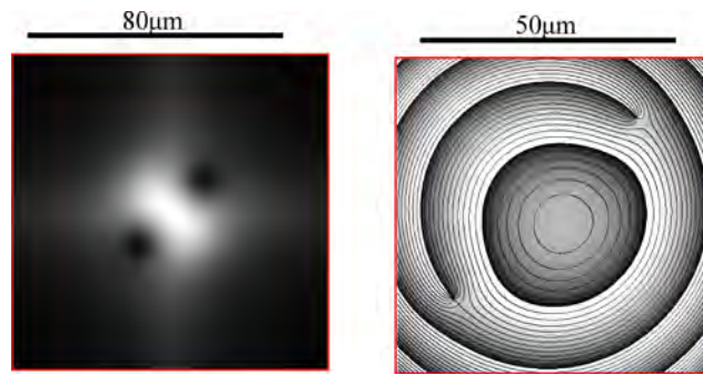
Fig. 7. Structurally stable topological dipole generated by the \pi -phase plate ( \alpha = \beta = 0 , w_0 = 30 \mu\text{m} and z = 50 \mu\text{m} ).
