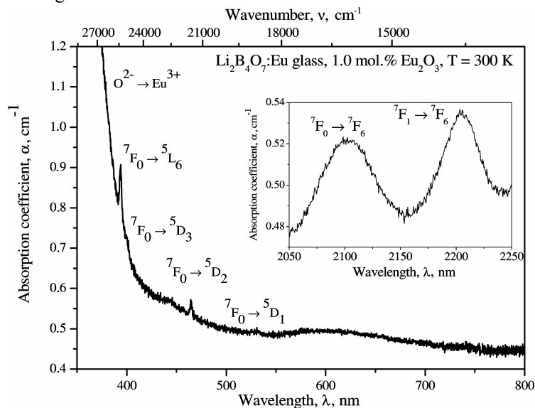
Fig. 1. Optical absorption spectrum for the Li 2 B 4 O 7 :Eu glass containing 1.0 mol. % Eu 2 O 3 , measured at T=300K.
