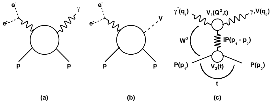
Fig. 1. Diagrams of DVCS (a) and VMP (b); (c) DVCS (VMP) amplitude in a Regge-factorized form
