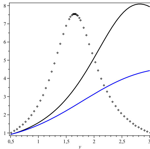
Fig. 4. Ratio \chi_{\text{Skyrme}}(y)/\chi_{\text{free}} (see (16), (18), and (19)) for SNM with generalized parametrizations (BSk18 points, BSk20 upper line, and BSk21 lower line) of the Skyrme forces [20, 21] and a spin-triplet p -wave pairing of the {}^3\text{He} – A type at T = 0 as a function of the reduced density y = n/n_0
