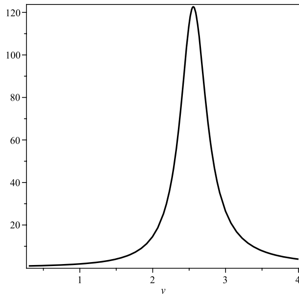
Fig. 3. Ratio \chi_{\text{BSk19}}(y)/\chi_{\text{free}} (see (17)) for SNM with generalized BSk19 parametrization [21] of the Skyrme forces and a spin-triplet p -wave pairing of the {}^3\text{He} – A type at T = 0 as a function of the reduced density y = n/n_0
