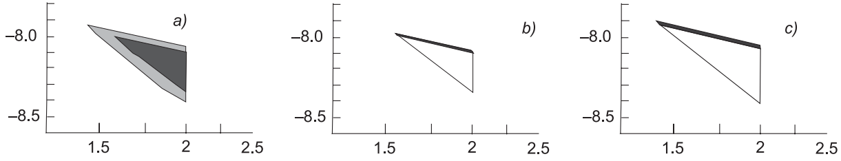
Fig. 12. Red region “DM” from Fig. 10 in the scaled-up form: a) \theta_{13} = 0^\circ type A (dark) and type B (light); b) type A: \theta_{13} = 0^\circ (white) and \theta_{13} = 10^\circ (black); c) type B: \theta_{13} = 0^\circ (white) and \theta_{13} = 10^\circ (black). The variable M/1 GeV is along the abscissa axis, and the variable \text{Log}_{10}(\Theta^+\Theta)_{22} is along the ordinate axis
