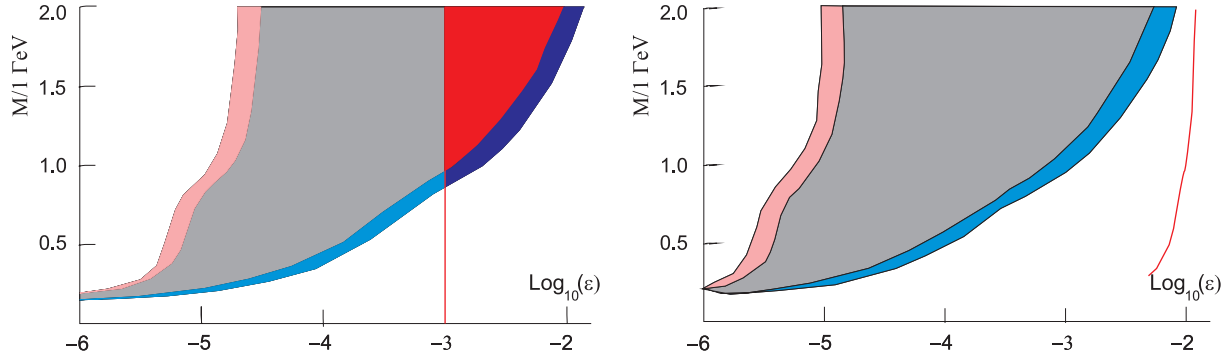
Fig. 10. Case of the inverted hierarchy: a) \theta_{13} = 0 , b) \theta_{13} = 10^\circ . The pink, grey, and red regions correspond to the A type of solutions. The grey, red, sky blue, and blue regions correspond to the B type of solutions. The points on these regions satisfy constraint (71). The region on the right from the red line satisfies also condition (1)
