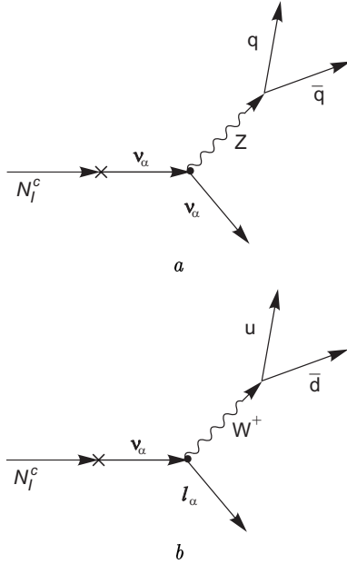
Fig. 1. Decay of a sterile neutrino via a Z -boson (a) and a W^+ -boson (b) (the cross on the line of a sterile neutrino means an oscillation of a sterile neutrino to an active one)
