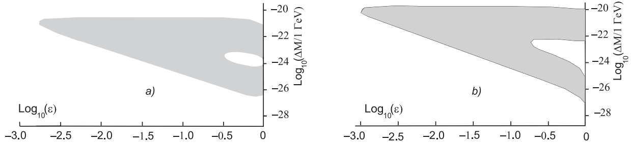
Fig. 7. Grey areas represent the regions of parameters, where 10^{-3} < \Delta < 2/11 for M = 1 GeV in case of the normal (a) and inverted hierarchies (b)
