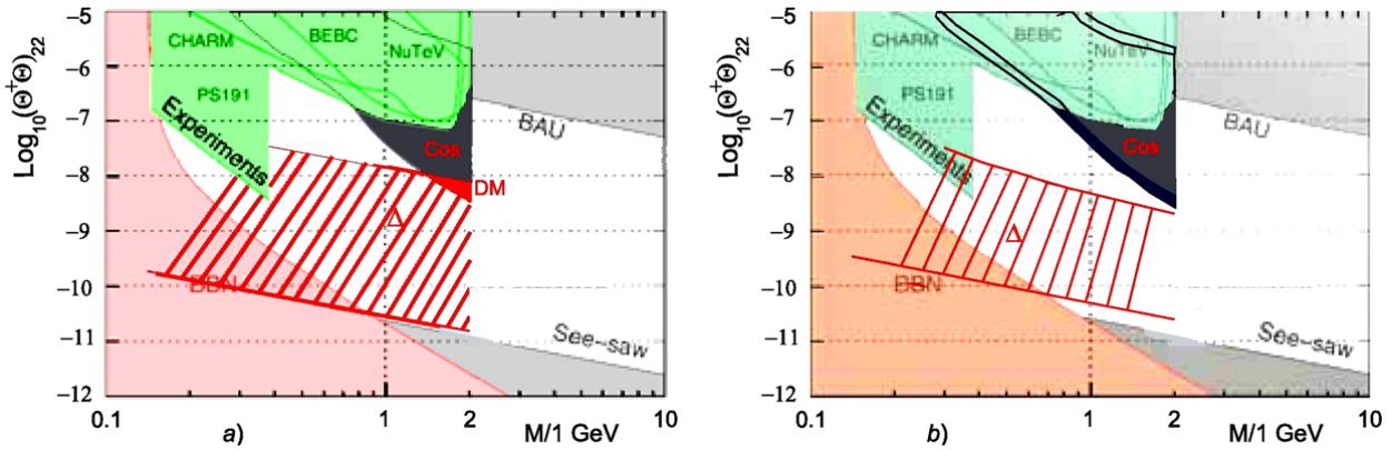
Fig. 11. Imposition of our constraints and summarized constraints from [23]: a) the case of the normal hierarchy, b) the case of the inverted hierarchy
