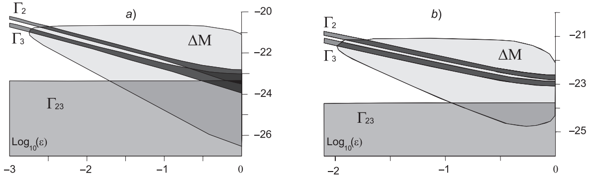
Fig. 8. Values of rates \text{Log}_{10}(\Gamma_I/1 \text{ GeV}) , \text{Log}_{10}(\Gamma_{23}/1 \text{ GeV}) , and \text{Log}_{10}(\Delta M/1 \text{ GeV}) for the leptonic asymmetry \Delta > 10^{-3} in the case of M = 1 \text{ GeV} and \theta_{13} = 10^\circ are on the ordinate axis: a ) is the case of the normal hierarchy (A type of a solution), and b ) is the case of inverted hierarchy (B type of a solution)
