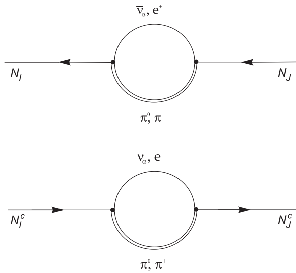
Fig. 4. Contributions to the effective Hamiltonian
