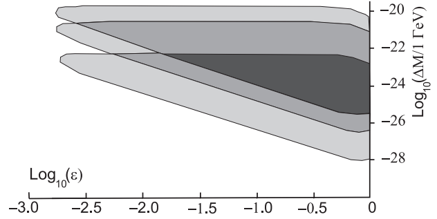
Fig. 5. Grey areas are the regions of parameters, where \Delta > 10^{-3} in the case of the normal hierarchy. The areas correspond to M = 0.3 GeV (bottom), M = 1 GeV (middle), M = 2 GeV (top)
