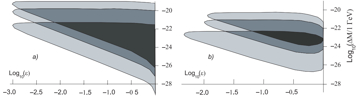
Fig. 6. Grey areas are the regions of parameters, where \Delta > 10^{-3} in the case of the inverted hierarchy. The areas correspond to M = 0.3 GeV (bottom), M = 1 GeV (middle), M = 2 GeV (top). Parts a) and b) represent the case of \theta_{13} = 0^\circ and 10^\circ , respectively
