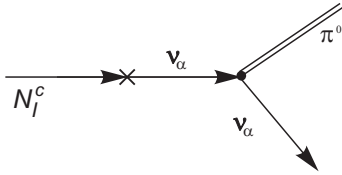
Fig. 2. Effective low-energy decay of a sterile neutrino into a \pi^0 meson and an active neutrino
