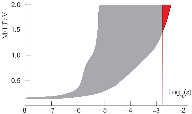
Fig. 9. Case of the normal hierarchy. The points on grey and red regions satisfy constraint (71). The region on the right from the vertical red line satisfies also condition (1)
