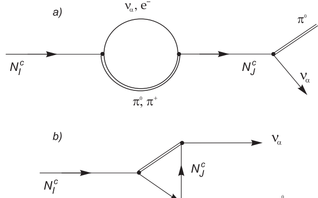
Fig. 3. Example of one-loop diagrams of the decay N_I \rightarrow \nu_\alpha \pi^0
