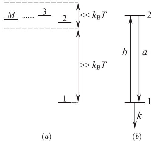
Fig. 1. A diagram of M energy levels (numbers) distinctly distant each other (in thermal energy units) (a) and its coarse-grained reduction by a two-level scheme with effective rate constants a , b , and k (b)
