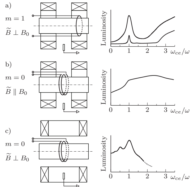
Fig. 1. Schematic diagram of experimental devices and experimental results
