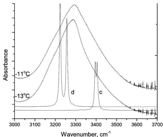
Fig. 6. Comparison of experimental FTIR spectra at -11 and -13\text{ }^{\circ}\text{C} with the calculated ones for a trimer ( c ) and a tetramer ( d ) in the O–H stretching region
