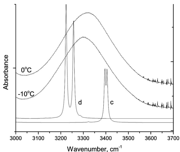
Fig. 5. Comparison of experimental FTIR spectra at 0 and -10\text{ }^{\circ}\text{C} with the calculated ones for a trimer ( c ) and a tetramer ( d ) in the O–H stretching region
