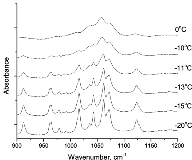
Fig. 2. Experimental FTIR spectra of n -nonan-1-ol for various temperatures in the spectral region 900 – 1200 \text{cm}^{-1}
