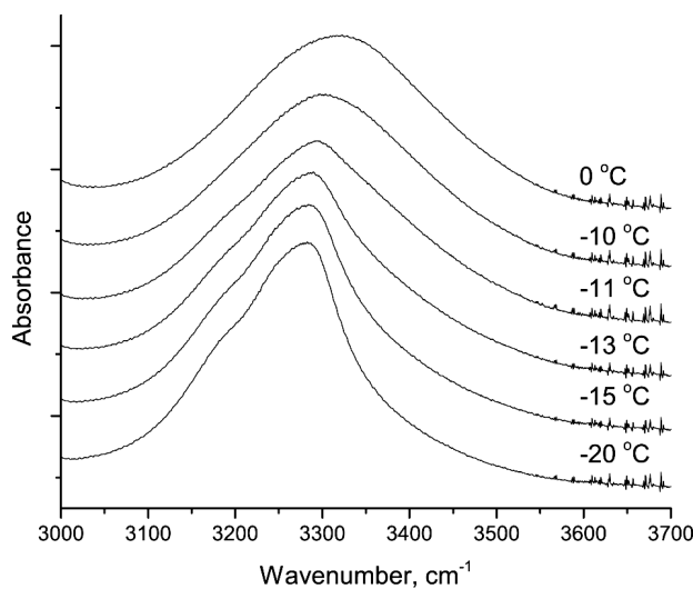
Fig. 3. Experimental FTIR spectra of n -nonan-1-ol for various temperatures in the spectral region 3000 – 3700 \text{cm}^{-1}
