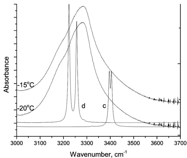
Fig. 7. Comparison of experimental FTIR spectra at -15 and -20\text{ }^{\circ}\text{C} with the calculated ones for a trimer ( c ) and a tetramer ( d ) in the O–H stretching region
