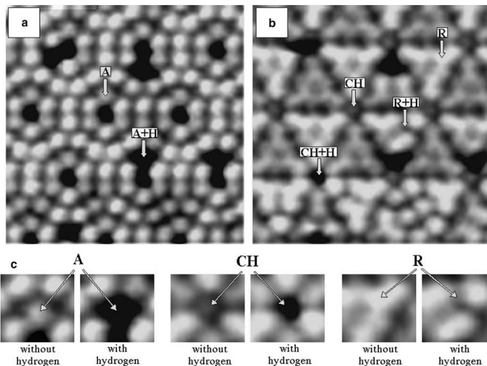
Puc. 12. Typical STM images of the same area on the H/Si(111) – 7 \times 7 surface at positive (1.2 V, 56 pA) (a) and negative (–1.2 V, 56 pA) (b) voltages on the specimen. Images were obtained, by using Bi/W tips. Places of hydrogen adsorption: adatom (A), residual atom (R), and corner holes (CH). The scaled-up variants of those images [37] (c)
