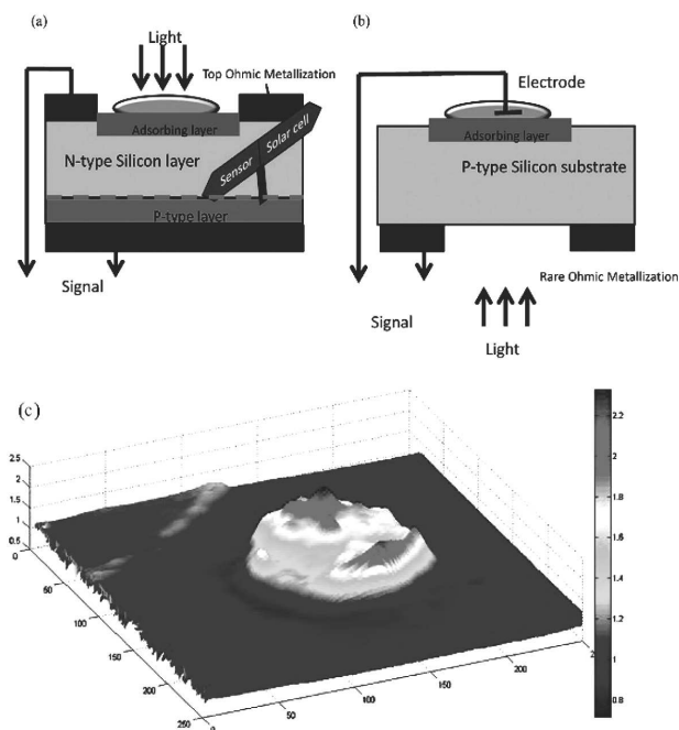
Puc. 10. Basic design of an “electronic tongue” on the basis of a photo-electric transducer (a, b) and the experimental 2D distribution of the induced current with a droplet of distilled water on the rear side of a p-n junction (c)
