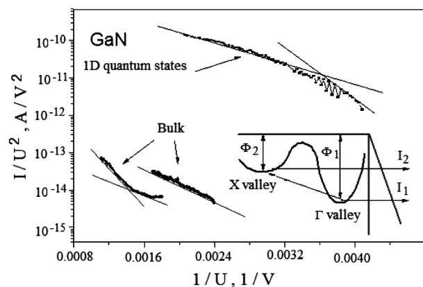
Puc. 2. Experimental I – V characteristics for electron field emission from GaN plotted in the Fowler–Nordheim coordinates
