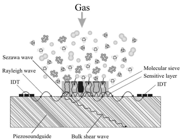
Puc. 14. Layered structure with a molecular sieve on the piezoelectric surface used as a gas sensor
