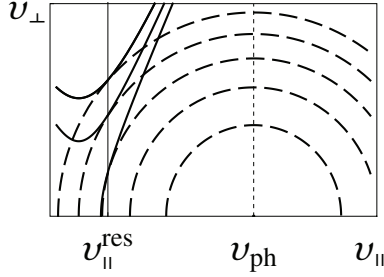
Fig. 1. Characteristics determined by the K&E equation (2) (dashed curves) and Eq. (20) (thick solid lines) in the (v_{\parallel}, v_{\perp}) space. In calculations, we took \tilde{\omega} = 1.2 and l = 1 , so that v_{\parallel}^{\text{res}}/v_{\text{ph}} = 1/6 according to (23)
