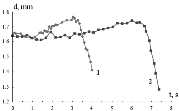
Fig. 3. Octadecane droplet size history: d = 1.64 mm, E = 0 kV/m (1), E = 82 kV/m, T_g = 720 K (2)
