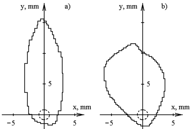
Fig. 1. Octadecane droplet burning: without electric field (a); in the electric field E = 82 kV/m (b)
