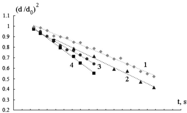
Fig. 2. Effect of a dc electric field on the burning rate of octadecane droplets: d = 1.96 mm, E = 0 (1), E = 82 kV/m (2); d = 1.64 mm, E = 0 (3), E = 82 kV/m (4)
