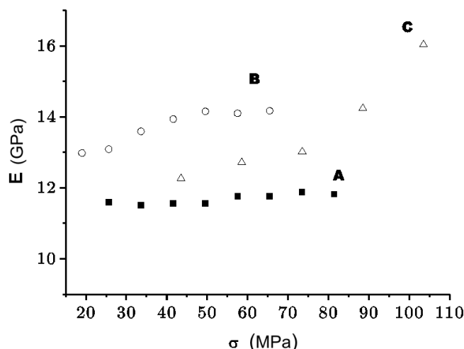
Fig. 2. Dependences of the elastic modulus on the loading, E(\varepsilon) , for various specimens: fibroin fiber obtained immediately from silkworm's glands (A), fibroin fiber obtained from silkworm's glands and treated in an alkaline solution (B), and fibroin fiber obtained from a silkworm cocoon (C)
