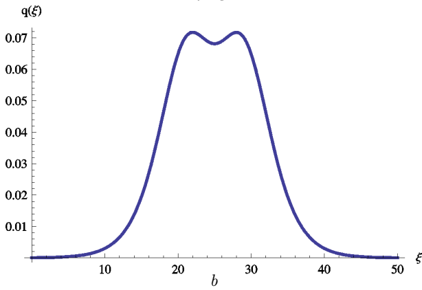
Fig. 3. Results of numerical simulations for the electron density (green dashed line) and the velocity distribution (red solid line) at \bar{U} = 60 (a). Blue curve corresponds to bisolectron density profile q(x) is based on the analytical results (64) at l = l_0 = 8 (b)
