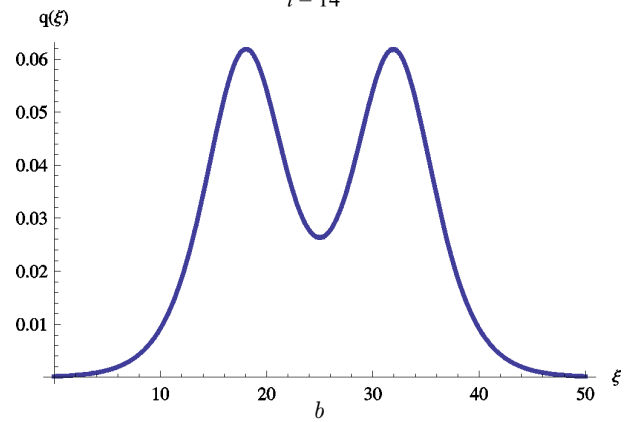
Fig. 4. Results of numerical simulations for the electron density (green dashed line) and the velocity distribution (red solid line) at \bar{U} = 100 (a). Blue curve corresponds to bisolectron density profile q(x) is based on the analytical results (64) at l = l_0 = 14 (b)
