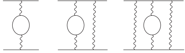
Photons exchange diagrams of eVP contributions
