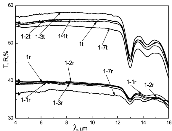
Fig. 4. IR transmission (t) and reflection (r) spectra of GaAs specimens: (1) raw specimen, (1-1) specimen 1 after the treatment in H^+ plasma (a discharge power of 175 W, a gas pressure of 0.8 Torr, a treatment time of 30 min), (1-2) specimen 1-1 after the HF treatment under a mask (a discharge power of 250 W, a gas pressure of 0.8 Torr, a treatment time of 62 min), (1-3) specimen 1-2 after the HF treatment under a mask (a discharge power of 250 W, a gas pressure of 0.8 Torr, a treatment time of 57 min), (1-7) specimen 1-3 after the microwave treatment for 10 min
