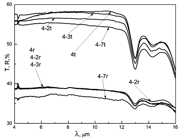
Fig. 2. IR transmission (t) and reflection (r) spectra of tellurium-doped GaAs specimens: (4) raw specimen, (4-2) specimen 4 after the HF treatment under a mask (a discharge power of 250 W, a gas pressure of 0.8 Torr, a treatment time of 62 min), (4-3) specimen 4-2 after the HF treatment under a mask (a discharge power of 250 W, a gas pressure of 0.8 Torr, a treatment time of 57 min), (4-7) specimen 4-3 after the microwave treatment for 10 min
