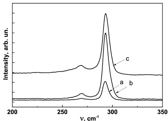
Fig. 1. Raman spectra of GaAs specimens: raw (a), No. 1 (b), and No. 4 (c). See Table for the specimen nomenclature
