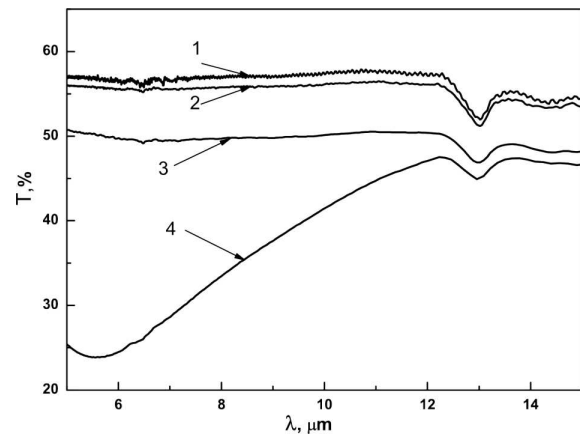
Fig. 3. IR transmission spectra of Cr-doped GaAs specimens [2]: (1) raw specimen, (2) specimen 1 after the HF treatment under a mask (a discharge power of 250 W, a gas pressure of 0.8 Torr, a treatment time of 15 min), (3) specimen 2 after the HF treatment under a mask (a discharge power of 250 W, a gas pressure of 0.8 Torr, a treatment time of 47 min), (4) specimen 3 after the annealing at 600 °C for 30 min in the argon atmosphere
