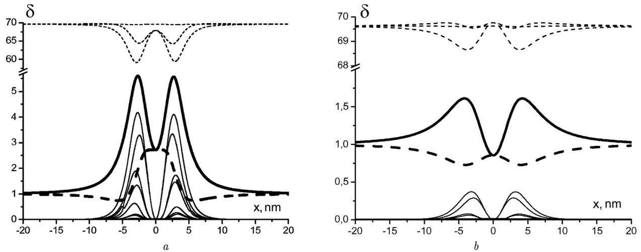
Fig. 4. Optical absorption enhancement as a function of the ring shift with respect to the center of a metal nanoparticle with small radius. Bold solid and dashed curves correspond to the states with l_k = \pm 1 and i = - , thin solid curves to transitions into other exciton states of the system, thin dashed lines to plasmon states. The external nanoshell radius R = 3 nm, the internal radius R_1 = 2.9 nm, \epsilon^{(0)} = 1.4 , \epsilon^{(2)} = 1 , and \hbar\Gamma = 0.1 eV. (a) The ring is located close up to the nanoparticle ( L = 0 ); (b) the distance between the nanoparticle surface and the ring plane L = 1.5 nm
