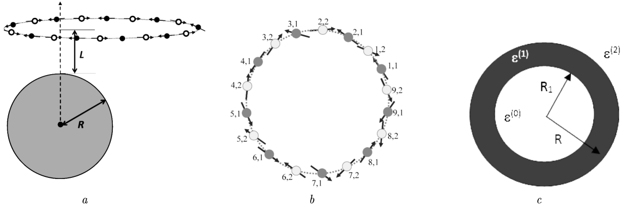
Fig. 1. Schematic diagram of the system consisting of a metal nanoparticle and the molecular ring B850 (a). Schematic diagram of the molecular ring B850 (b). Arrows designate the dipole moments of the molecules in the ring. Metal nanoshell with a dielectric core (c)
