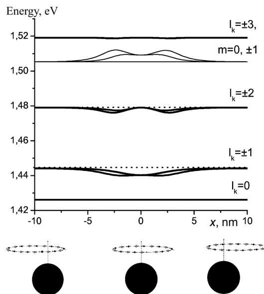
Fig. 3. Energies of some lowest states in the system as functions of the ring shift with respect to the center of a metal nanoparticle of the radius R = 3 nm for the parameters \varepsilon^{(0)} = 1.4 , \varepsilon^{(2)} = 1 , \hbar\Gamma = 0.1 eV, L = 0 , and the internal radius R = 2.9 nm. Bold curves correspond to exciton states, thin curves to plasmon states, branches j, i = - . Dotted lines exhibit the levels of an isolated molecular ring
