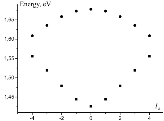
Fig. 2. Exciton spectrum of a molecular ring with N = 18 . Circles and squares denote states with i = + and i = - , respectively
