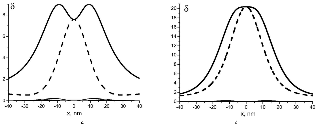
Fig. 5. Optical absorption enhancement as a function of the ring shift with respect to the center of a metal nanoparticle with large radius. Bold solid and dashed curves correspond to the states with l_k = \pm 1 and i = - ; excitation of other exciton states of the system (thin solid curves) are much less probable; curves corresponding to plasmon states are not shown. The external nanoshell radius R = 20 nm, \epsilon^{(0)} = 1.4 , \epsilon^{(2)} = 1 , \hbar\Gamma = 0.1 eV, the distance between the nanoparticle surface and the ring plane L = 1.5 nm, the internal radius R_1 = 19.3 (a) and 19.4 nm (b)
