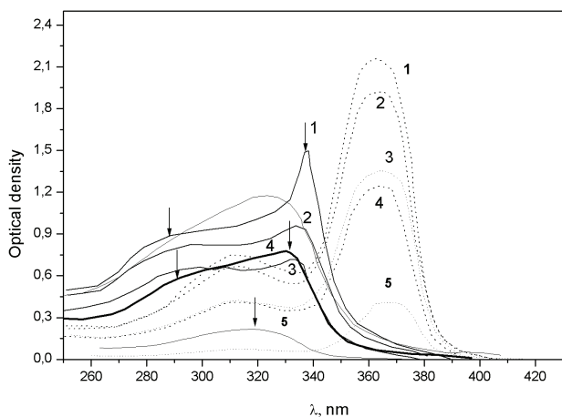
Fig. 2. Thickness dependence of the absorption spectra of a PDHS film at 293 K (dotted line) and at 318 K (solid line). Arrows indicate the maxima of new bands at 337 and 287 nm with decreasing the film thickness. Numbers show the spectra of the same thickness
