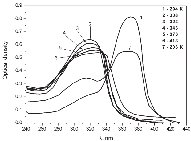
Fig. 7. Temperature dependence of the PDHS absorption spectra with M_{w2} at the second thermal cycle
