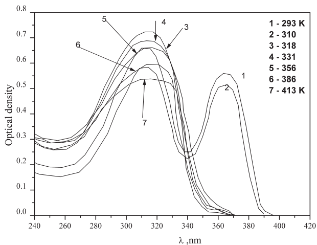
Fig. 8. Temperature dependence of the PDHS absorption spectra with M_{w3} at the heating from 293 to 413 K
