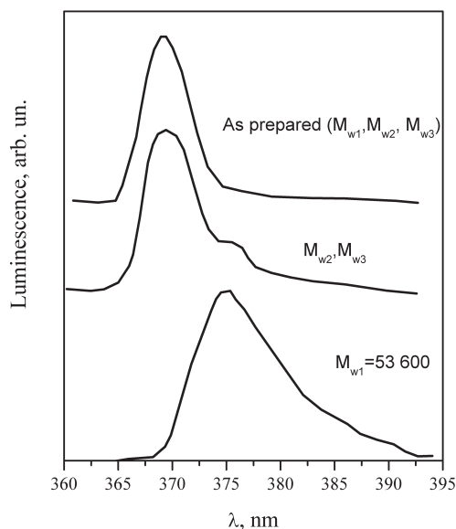
Fig. 4. Luminescence spectra of as-prepared PDHS films and thermally treated films with different molecular weights M_{wi} cooled down to room temperature ( T = 5 K, \lambda_{ex} = 313 nm)
