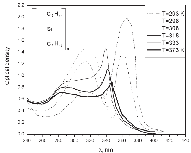
Fig. 1. Temperature dependence of the absorption spectra of PDHS films ( M_{w1} ) at the heating in the interval 293–373 K. Inset shows the PDHS structural formula
