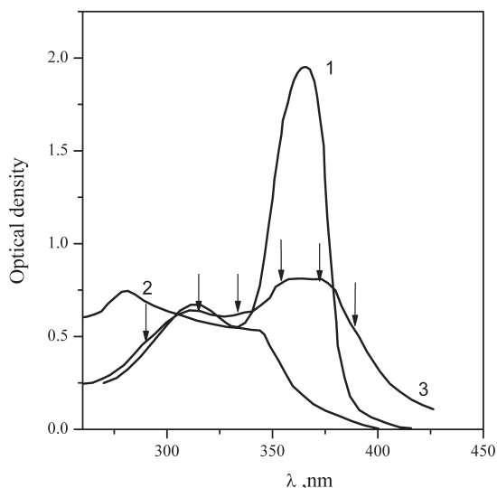
Fig. 3. Absorption spectra of a PDHS film: 1 – as-prepared at 293 K, 2 – after the heating to 398 K; 3 – after the heating to 398 K and the consequent cooling to 293 K. Arrows indicate the new bands arisen in the absorption spectra of films cooled to 293 K after the preliminary heating
