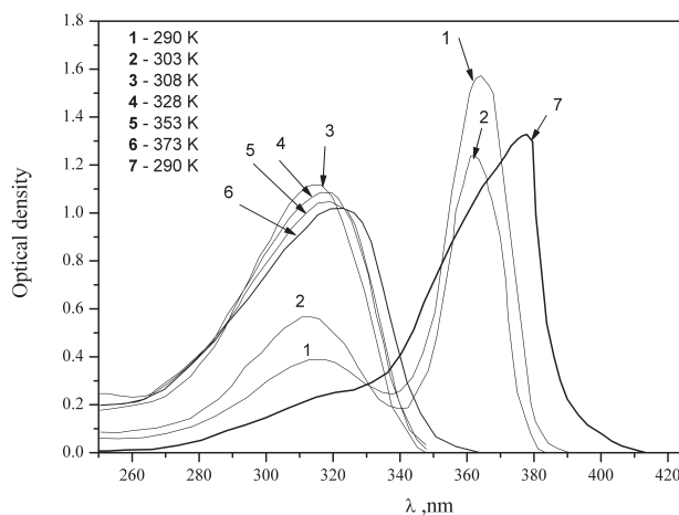
Fig. 6. Temperature dependence of the PDHS absorption spectra with M_{w2} at the first heating from 293 to 373 K
