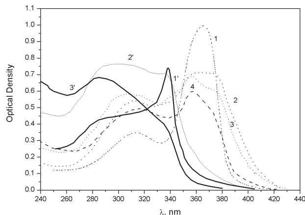
Fig. 5. Dependence of the absorption spectra of a PDHS film ( M_{w1} ) on the number of thermal cycles at 318 K (1, 2, 3, 4). Dashed lines indicate the absorption spectra: 1 – as-prepared film, 2, 3, 4 – the film cooled down to room temperature after the first, second, and third cycles
