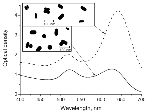
Fig. 1. Optical density spectra of a gold nanorod water suspension. Dashed line is the spectrum of the initial sample (before the femtosecond laser irradiation). Solid line is the spectrum of the sample after the long-term femtosecond laser irradiation. Insets show the corresponding TEM images of gold nanorods. Scale bar at each inset shows 100 nm
