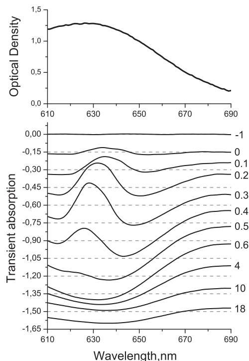
Fig. 5. Upper figure: Absorption spectrum of longitudinal plasmon mode. Lower figure: Transient absorption spectra measured at different time delays after the excitation by femtosecond laser pulses at 800 nm. The spectra are shifted vertically for clarity of presentation. Numbers on the right indicate the time delay in picoseconds between the pump and probe pulses
