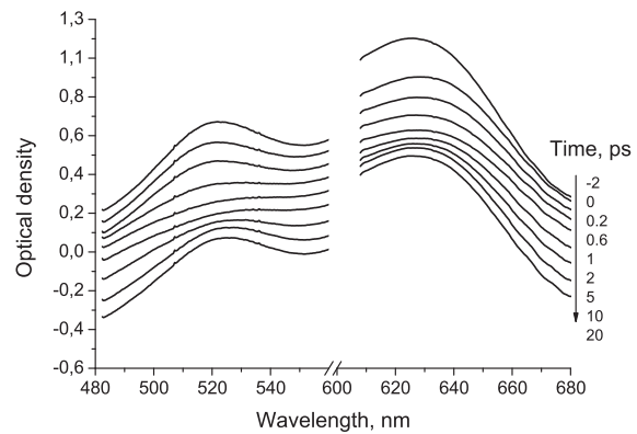
Fig. 2. Evolution of the both longitudinal (peak at 520 nm) and transverse (peak at 630 nm) plasmon absorption bands of gold nanorods after the femtosecond laser irradiation at 400 nm. The spectra are shifted vertically for clarity of presentation. Numbers on the right indicate the time delay in picoseconds between the pump and probe pulses
