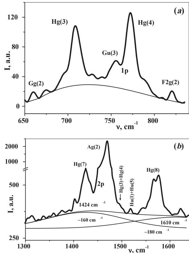
Fig. 5. Subtraction of vibrational induced local electronic bands (EB) in the Raman spectra of nanofilms of fullerene C_{60} in the case of the hot (a) and cold (b) methods of deposition and polymerization by diamine in the field of vibrational bands Hg(3,4) (a) Ag(2), Hg(7,8) (b)
