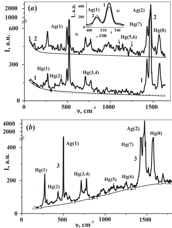
Fig. 1. Extraction of the wide electronic bands (EB) in the Raman spectra of C_{60} nanofilms with thicknesses of about 200 nm under hot (1) and cold (2) deposition processes (a) and microfilms with a thickness of 2 microns (b). The inset shows the Raman bands of breathing vibration Ag(1) and Si of crystalline silicon substrates for a C_{60} nanofilm
