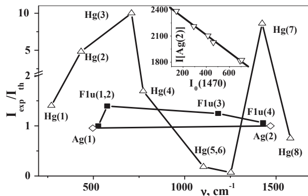
Fig. 6. The comparison of observed and calculated intensities of the Raman active Hg( j ) bands (open symbols) and IR \text{F}_{1u}(1-4) bands (dark symbols) ( b ). The inset shows the peak intensity decrease for Ag(2) band as a function of I_0(1470) in a vicinity of the current vibration
