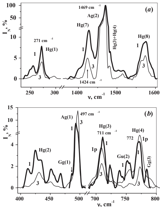
Fig. 2. Comparison of the vibrational bands normalized on line Ag(2) in the Raman spectra of nanofilms of fullerene C 60 fabricated by the hot method of deposition (1), microfilms of fullerene C 60 2 microns in thickness (3), and nanofilms polymerized by diamine (1p) in the region of the bands Hg(1), Ag(2) and Hg(7,8) and bands Hg(2,3,4) and Ag(1) (b)
