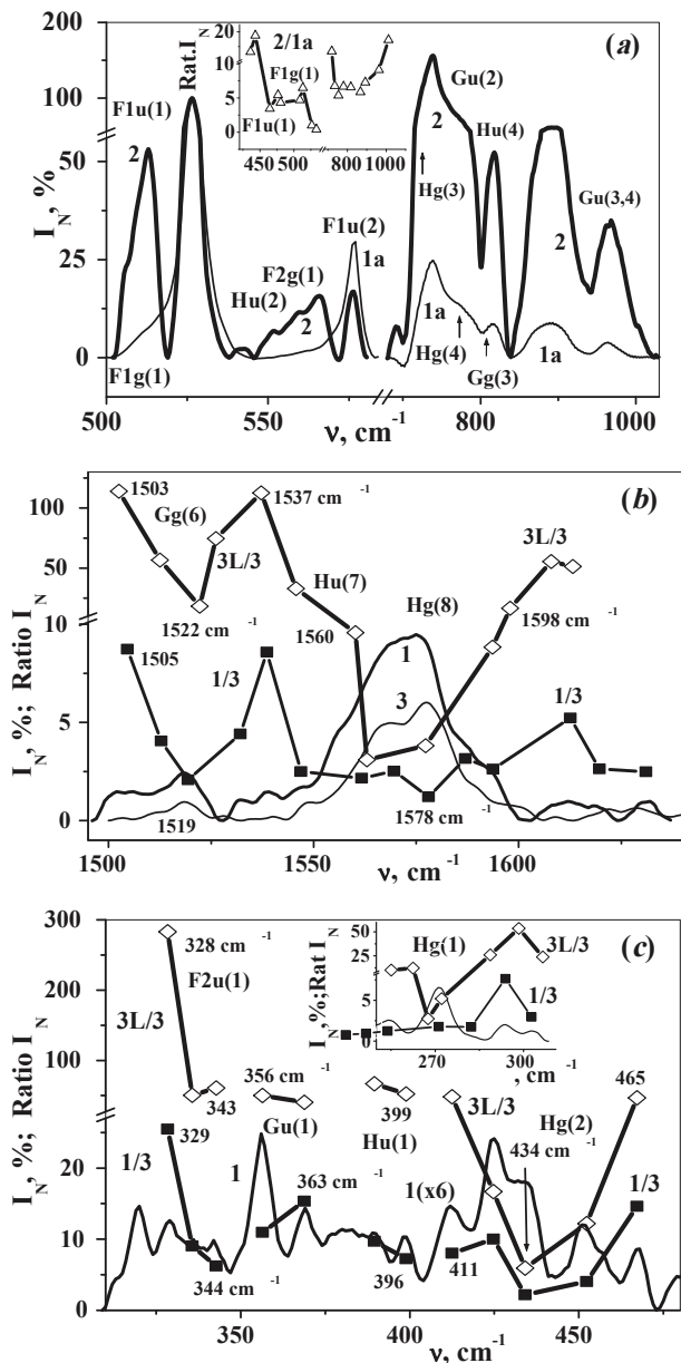
Fig. 4. The fragments of enhanced normalized IR absorption spectra (a) and Raman spectra (b, c) of the nanofilms of fullerene and the enhancement of the intensity of some “silent” and active vibrations in the vibrational spectra of nanofilms (curves with dark symbols), and microfilms after intense light irradiation (curves with open symbols) in comparison with the initial microfilms (a, b, c)
