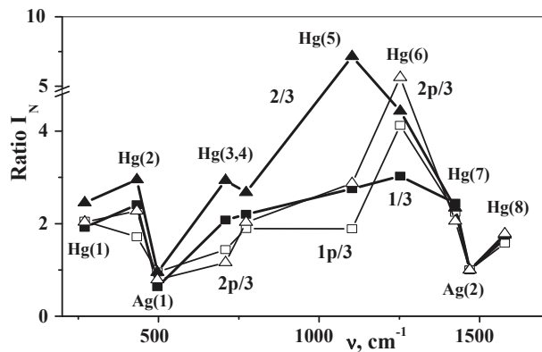
Fig. 3. Enhancement of active vibrations Hg(1–8) in the Raman spectra of the nanofilms of fullerene C 60 in comparison with microfilms about 2 microns in thickness in the cases of the hot (1/3) and cold (2/3) deposition methods, as well as nanofilms polymerized by diamine (1/3 and 2p/3)
