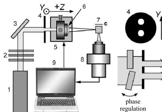
Fig. 1. Schematic diagram of the experimental installation: regenerative amplifier Legend F-1K-HE (1), neutral filters (2), rotary mirror (3), diaphragm (4), coordinate stage (5), objective lens (6), specimen (7), microscope objective and CCD-chamber (8), and personal computer (9)
