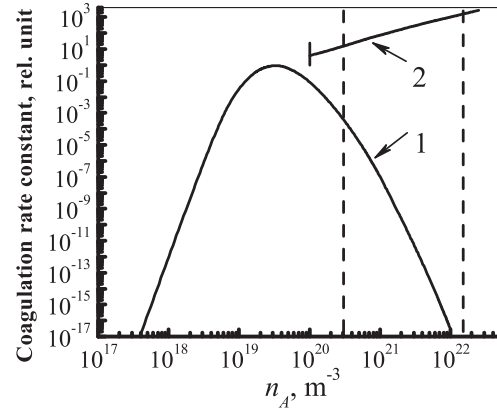
Fig. 5. The dependence between the relative coagulation rate and the concentration of potassium atoms in the plasma of products of the combustion of Al with additive \text{K}_2\text{CO}_3 : 1 – the coagulation rate of charged particles; 2 – the coagulation rate with the regard for the of interaction of particles in a plasma [11]
