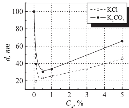
Fig. 3. Size of \text{Al}_2\text{O}_3 particles vs. the additive concentration in the initial fuel (points – experiment; dashed line is an approximation)
