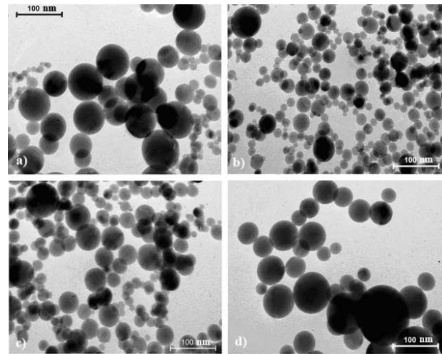
Fig. 2. Microphotographs of \text{Al}_2\text{O}_3 nanoparticles (magnification X 100 000): The concentration of an additive in the initial fuel contains: 0.1% \text{K}_2\text{CO}_3 (a); 0.5% \text{K}_2\text{CO}_3 (b); 1.0% \text{K}_2\text{CO}_3 (c); 5.0% \text{K}_2\text{CO}_3 (d)
