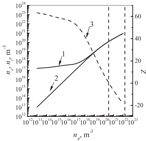
Fig. 4. Ionization equilibrium in the plasma of Al with K_2CO_3 additives; C_{Al} = 0.4 \text{ kg/m}^3 and r_{30} = 50 \text{ nm} . The vertical dashed lines mark the experimental region of the additive concentration; 1 – the concentration of electrons n_e , 2 – the concentration of ions, 3 – charge of the growing oxide nanoparticles Z
