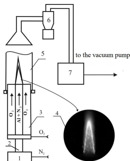
Fig. 1. Experimental setup: 1 – powder spraying unit; 2 – burner inner cylinder; 3 – burner outer cylinder; 4 – dust flame; 5 – moving tube to protect the flame; 6 – system for collecting the combustion products; 7 – fabric filter for collecting the combustion products
