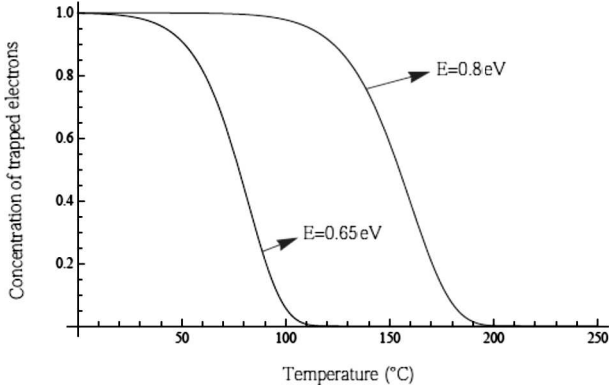
Fig. 2. Normalized concentration of electrons n_1(T) and n_2(T) in the first trap ( E_1 = 0.65 eV) and the second one ( E_2 = 0.8 eV) versus the temperature T (in ^{\circ}\text{C} ) for the first-order kinetics with the following values of parameters: n_1(0) = n_2(0) = 10^{15} \text{ cm}^{-3} , \beta = 1 \text{ }^{\circ}\text{C/s} , s_1 = s_2 = 10^8 \text{ s}^{-1}
