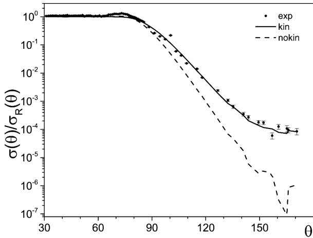
Fig. 5. Experimental data for the ^{16}\text{O} + ^{208}\text{Pb} elastic scattering at a beam energy of 95 MeV (Exp) [42] and the results of calculations in the framework of the optical model with the use of the nucleus-nucleus potential obtained both taking (kin) and not taking (nokin) the kinetic energy contribution into account
