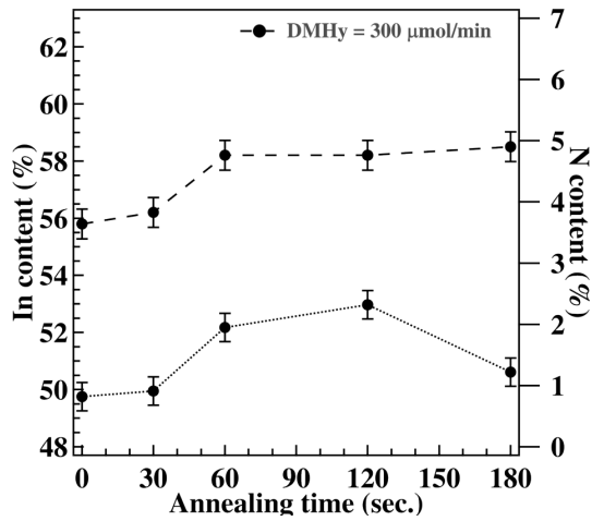
Fig. 4. In and N contents as functions of the annealing time for InGaPN alloy films
