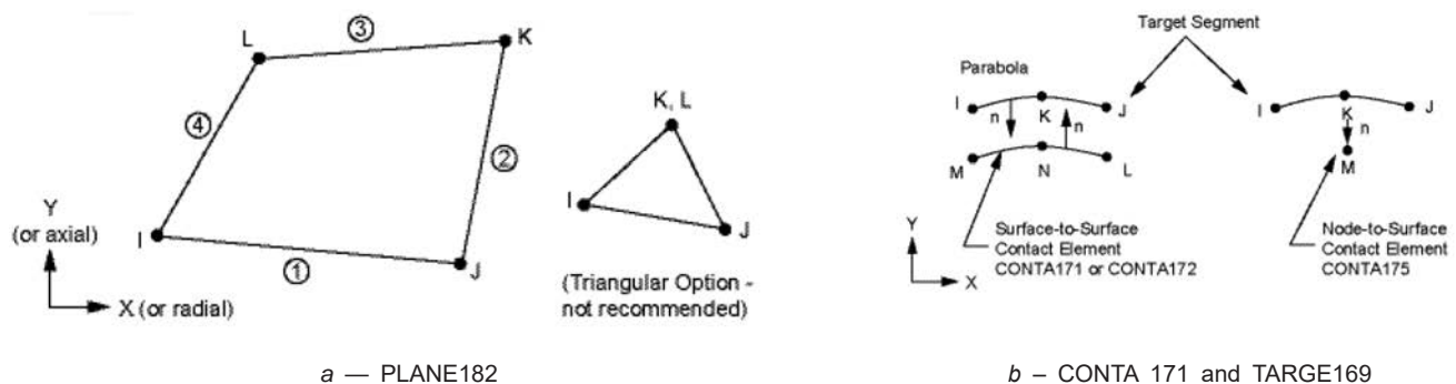
Fig. 2. PLANE182, CONTA 171 and TARGE169 geometry
