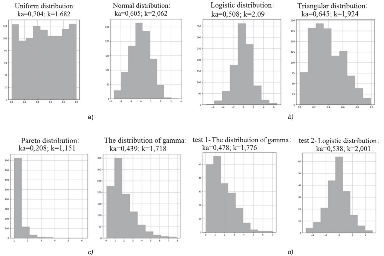
Fig. 2. Histograms of the generated samples of random variables with different distribution laws, where ka is the antokurtosis; k is the entropy coefficient of the distribution law
