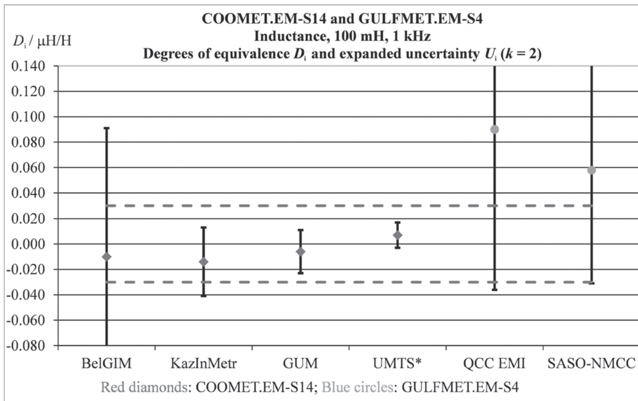
Fig. 11. DoE of NMIs in COOMET.EM-S14 and GULFMET.EM-S4 SCs in terms of RV_{S14}
