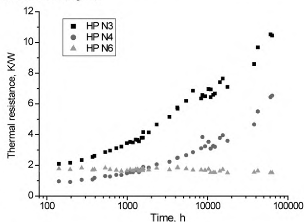
Fig. 3 – Change of the thermal resistance of heat pipes made of stainless steel with steel and copper fiber capillary structures with time
