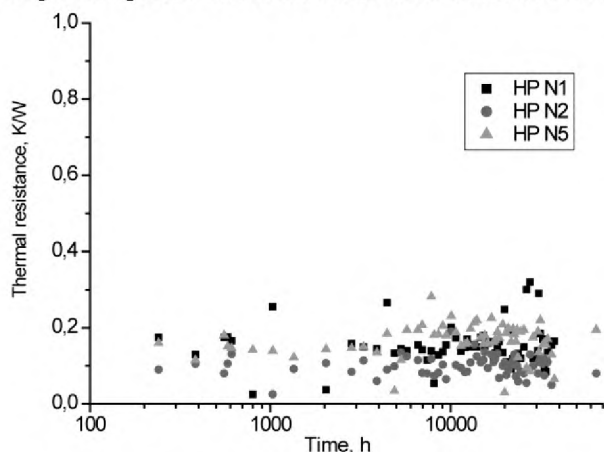
Fig. 2 – Change of the thermal resistance of the copper heat pipes with copper fiber capillary structures with time
