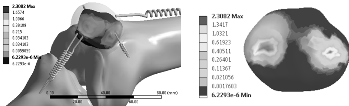
Fig. 2. Distribution by Mises equivalent stress in MPa patellar cartilage normally at 30° knee flexion, the trochlear dysplasia type A
