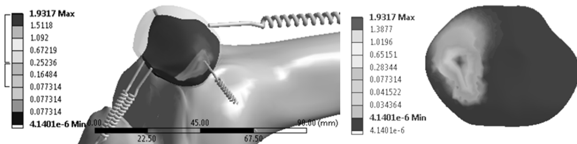
Fig. 3. Distribution of Mises equivalent stresses in MPa cartilage patellar instability at 30° knee flexion
