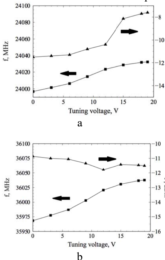
Fig. 5. Output power and frequency versus tuning voltage of push-push VCOs with second harmonic output at 24 GHz (a) and third harmonic output at 36 GHz (b).
