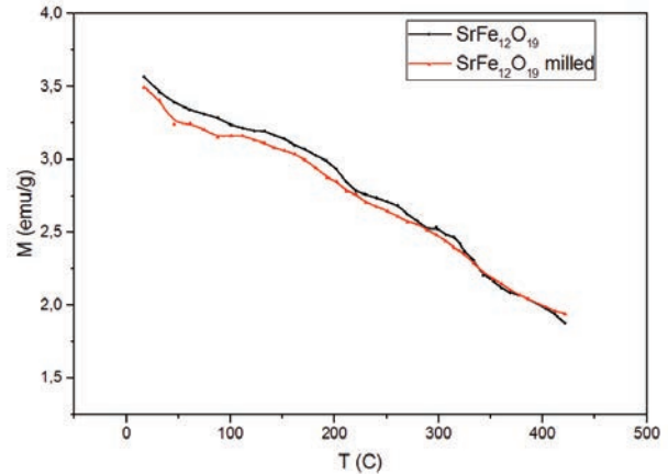
Fig.7. Temperature dependence of magnetization at constant external field H=1 kOe.
