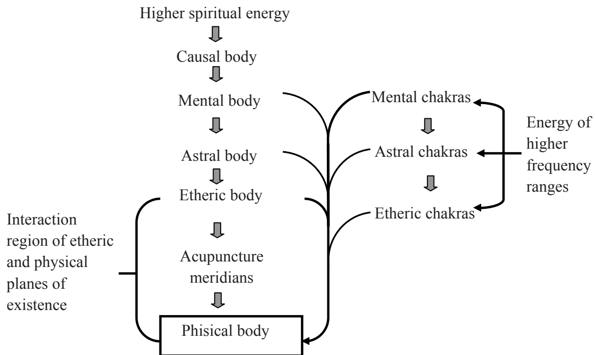
Scheme 3. A multidimensional human energy system
