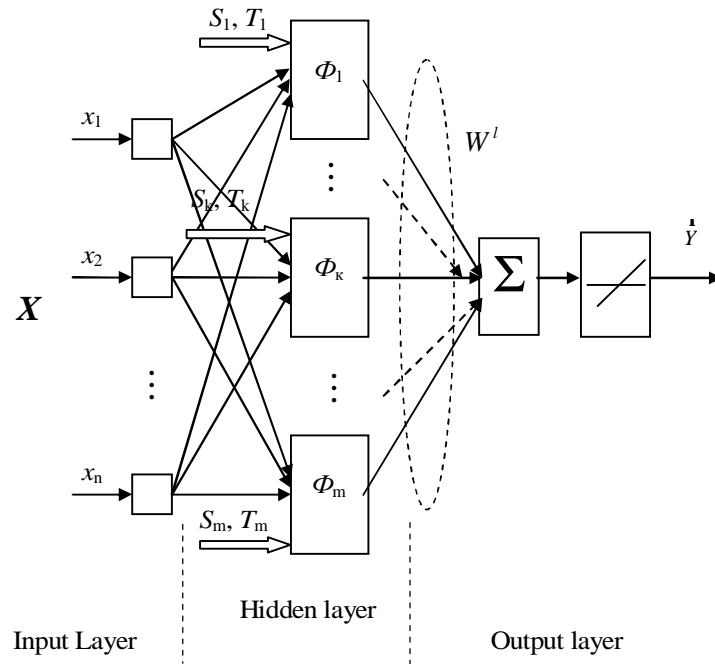
Fig. 2. Generalized architecture of wavelet neural network for solving classification
