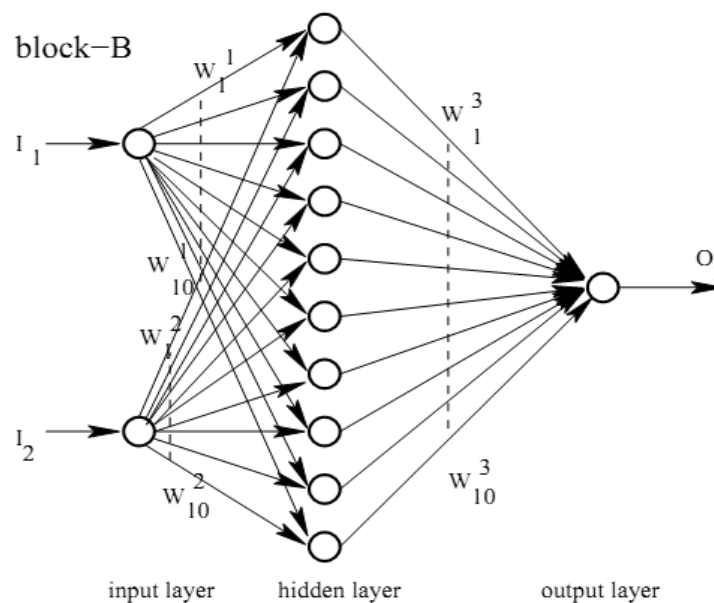
Fig. 2. Neural network
