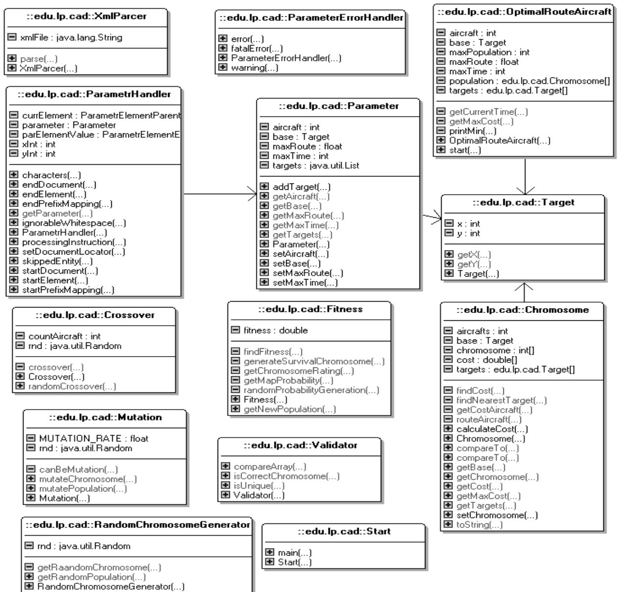
Fig. 5. The diagram of genetic algorithm classes
