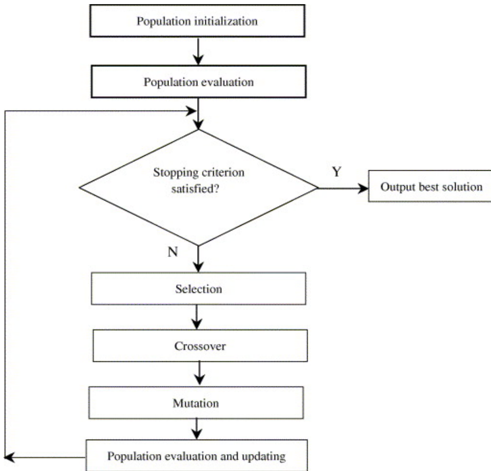
Fig. 3. Genetic algorithm work schema
