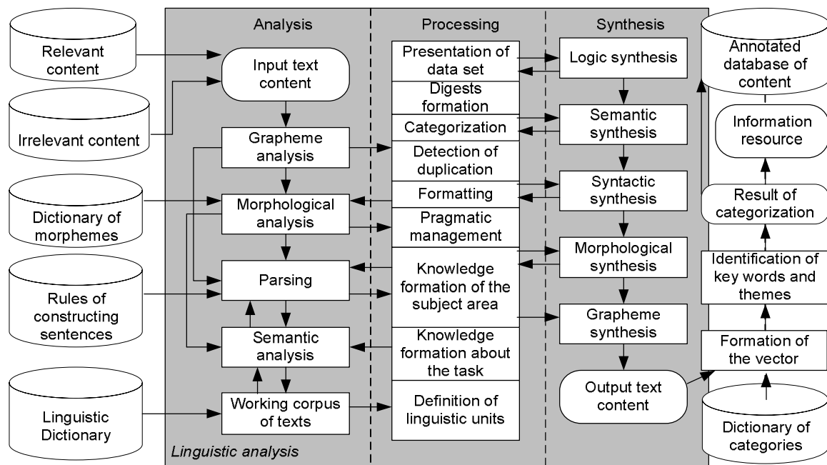
Fig. 1. Block diagram of the linguistic analysis of text content in the formation content
