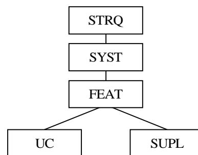
Fig. 3. Traceability requirements in Requisite Pro
