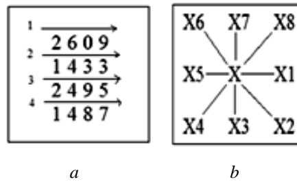
Fig. 2 and 2b. Direction and order numbers for comparison matrix
