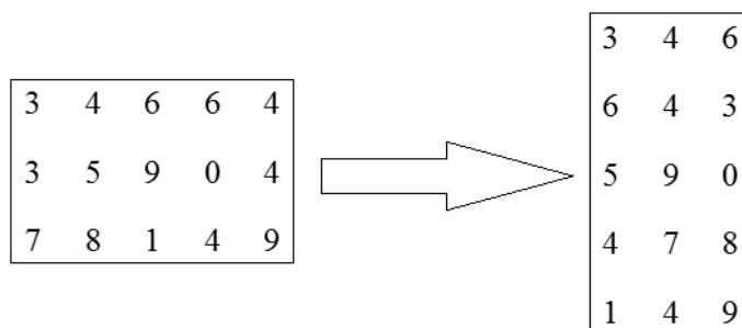
Fig. 9. Example conversion of input matrix inverse
