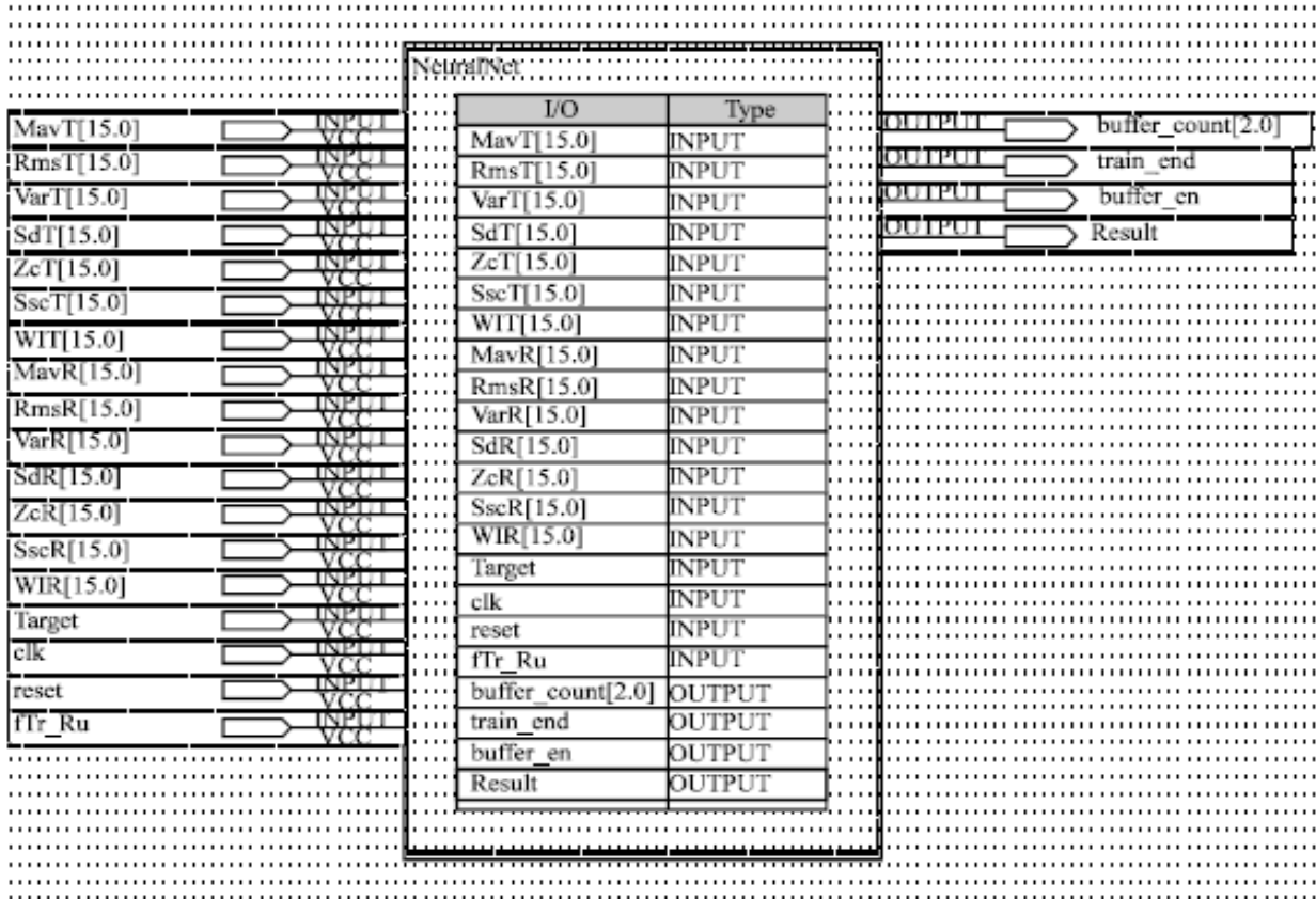
Fig. 2. Top entity for VHDL model of the network
