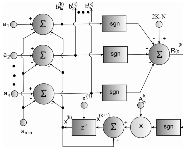
Fig. 1. Functional block diagram of discrete-time neural circuit presented in [1, 2]
