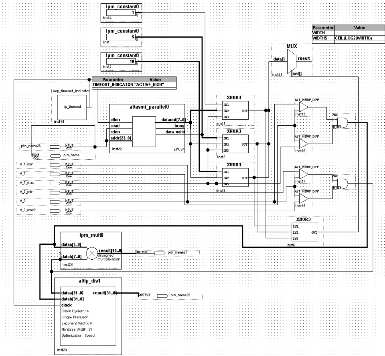
Fig.4. Hardware-description design of functional block diagram of discrete-time KWTA neural circuit presented in [21, 22]
