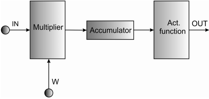
Fig. 3. Multiplier/accumulator architecture
