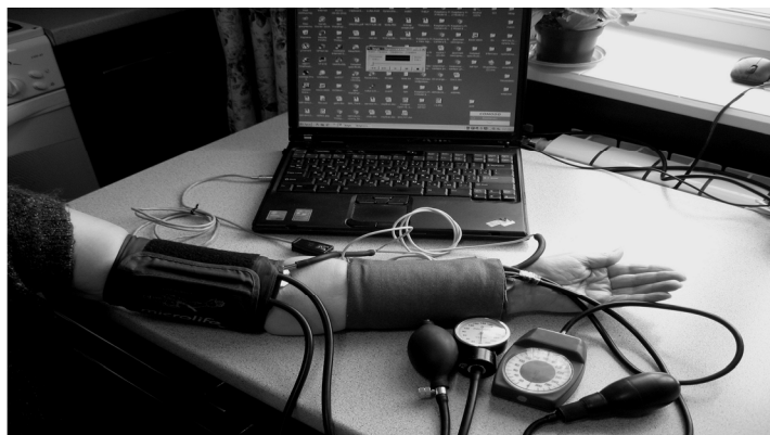
Fig. 5. Determination of the rate of pulse wave propagation
