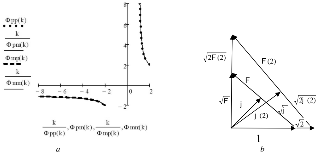
Fig.2.3. a – the graphs of functions Fsq(k) = \begin{cases} F_{pp} = 0.5(+k + L), & F_{mp} = (-0.5k + L), \\ F_{pm} = 0.5(+k - L), & F_{mm} = (-0.5k - L), \end{cases} L = \sqrt{\frac{k^2}{4} - k} ;
