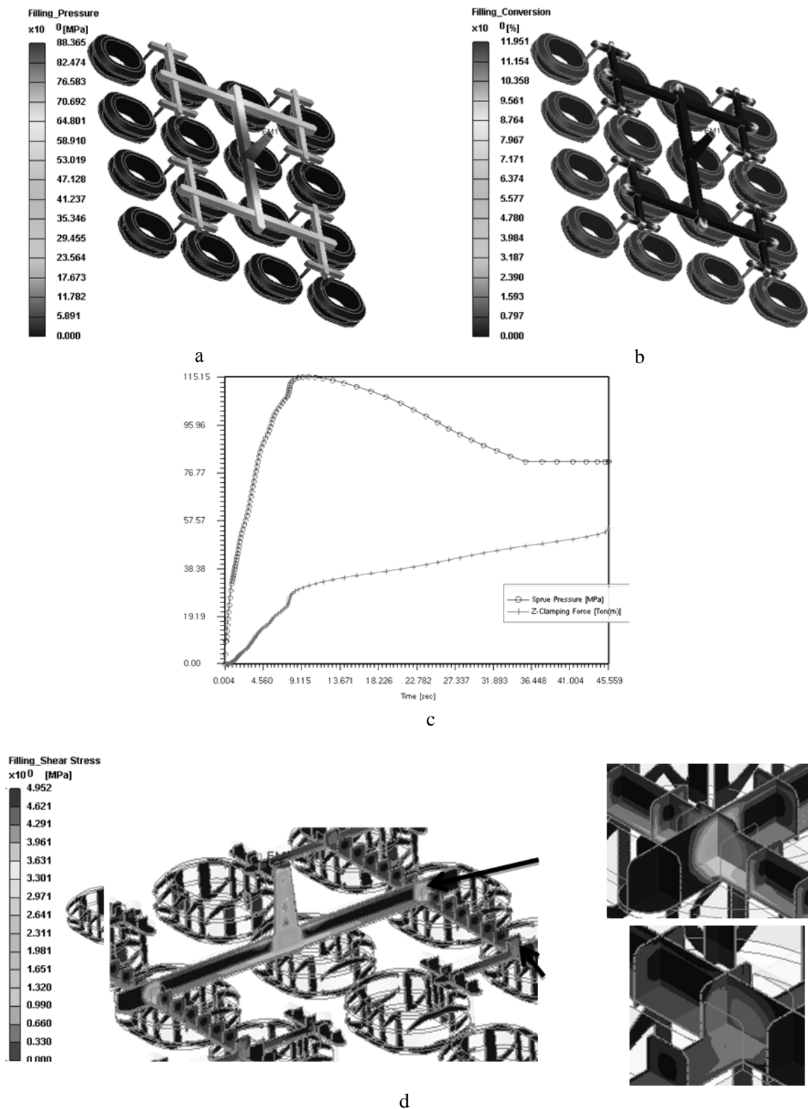
Fig. 2. The distributions for standard runner system: a – the injection pressure; b – crosslinking during filling; c – the injection pressure and the clamping force; d – the shear stress in the cross-sections
