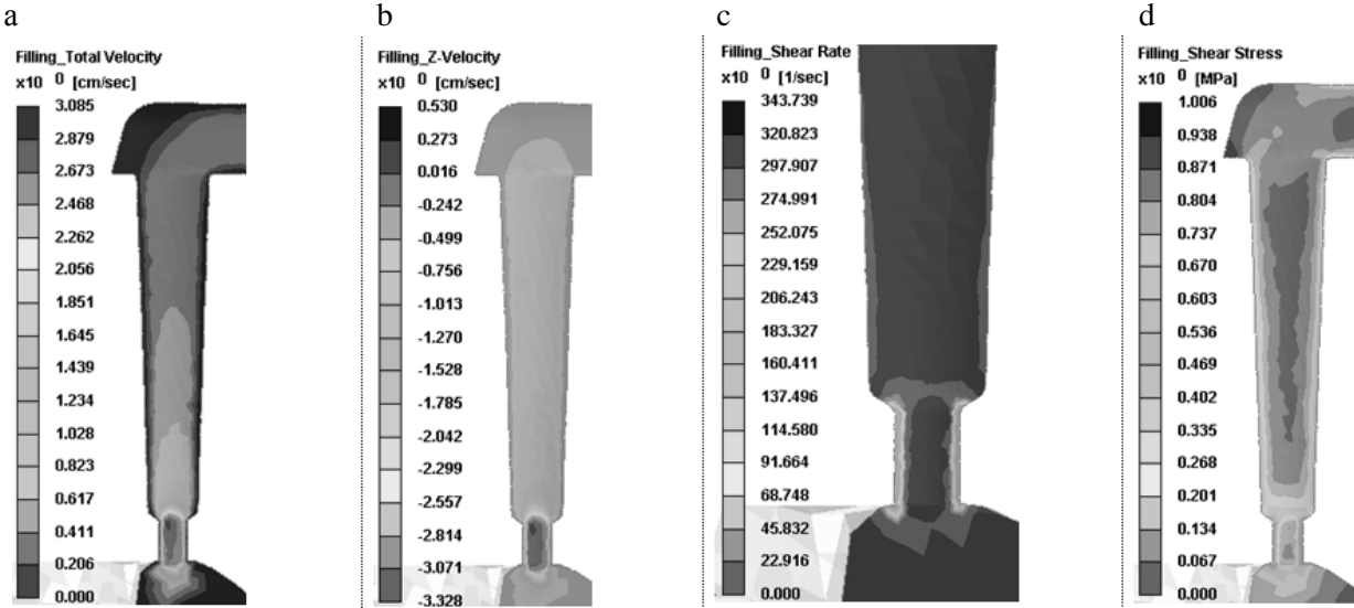
Fig. 5. Images: a – the flow rate; b – the vertical velocity; c – the shear rate, d – the shear stress
