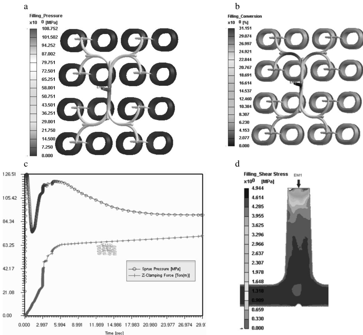
Fig. 4. The distributions for the modified system: a – the injection pressure; b – the crosslinking during filling; c – the injection pressure and the clamping force; d – shear stress in the sprue
