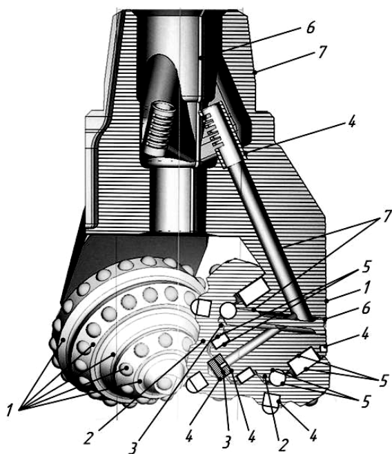
Fig. 1. Structure of three-cone rock bit with inserted hard-alloyed rock-destruction and protecting equipment, in which the chief components are marked. For these components such functionally-operating and technological requirements are placed as: 1 – wear resistance under conditions of hydro-abrasive and percussion-abrasive influences; 2 – resistance to plastic deformation and fracture failure; 3 – wear resistance under conditions of sliding friction and high contact temperatures; 4 – security of connection; 5 – contact endurance and wear resistance under conditions of rolling friction; 6 – high welding ability; 7 – high machining ability
