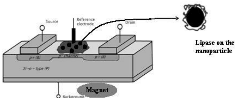
Fig. 5. Schematic representation of the ISFET with nanoparticles and a magnet [30]
