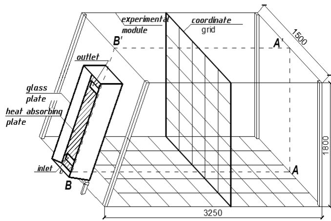
Fig. 2. Scheme (a) and photo (b) of experimental module
