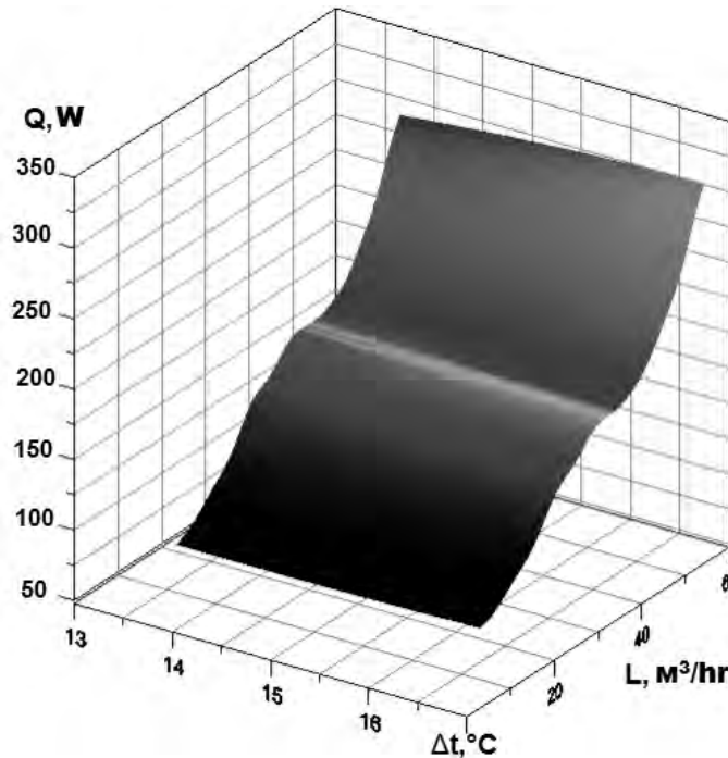
Fig. 4. Dependence the power of thermosyphon heliocollector, Q , W, from the temperature difference of cold air in the experimental modules and heated air after heliocollector, \Delta t , ° C, and it's volumetric flow rate, L , m 3 /hr
