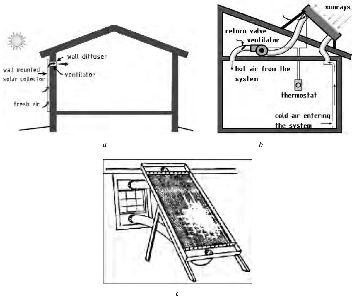
Fig. 1. Options for installation of solar air heaters: on the wall, b) on the roof, c) in the yard
