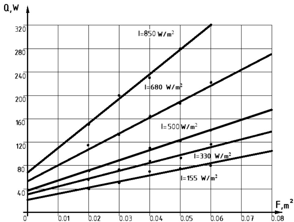
Fig. 3. Dependence the power of thermosyphon solar collector, Q , W , changes in the area of inlet and outlet of heliocollector, F , \text{m}^2 , and the intensity of heat flow, I , \text{W/m}^2
