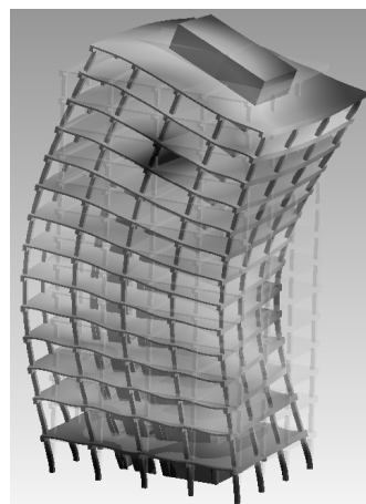
(f_{0(5)} = 6,8502 Hz) 5. Oscillation shape
