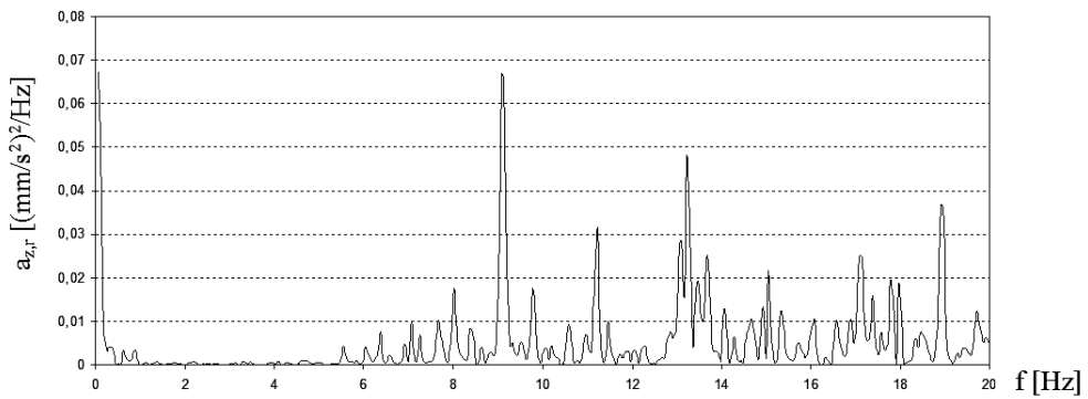
Fig. 14. PSD vibration acceleration (GM1M1(f)) in M1 – X
