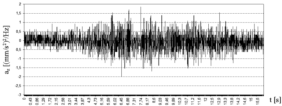
Fig. 13. Time record of vibration acceleration in M1 – X, RMS = 0,4341
