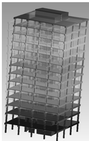
(f_{0(1)} = 1,3772 Hz) 1. Oscillation shape
