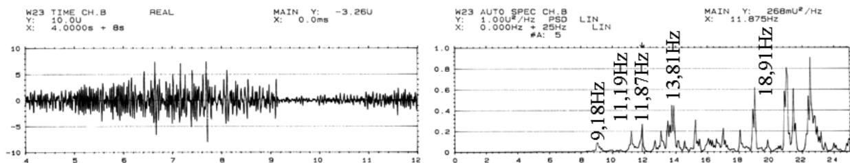
Fig. 2. Vibration acceleration time history at point M1, power spectral density (GM1M1 (f)) at point M1 – direction Z
