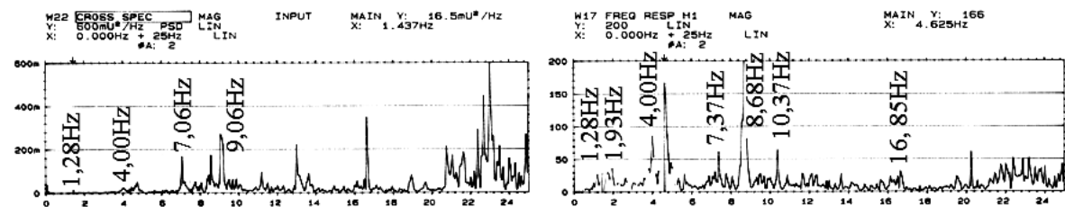
Fig. 7. Cross power spectral density (GM1M3 (f)), at points M1, M3 transfer characteristic (HM1M3 (if)), points M1, M3 – direction X
