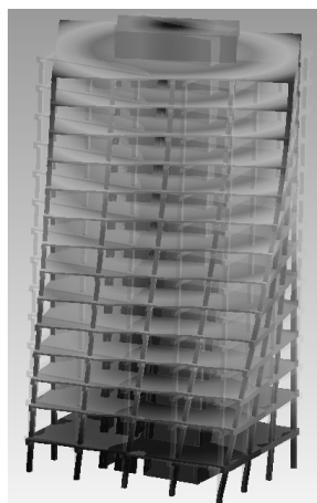
(f_{0(3)} = 3,3229 Hz) 3. Oscillation shape
