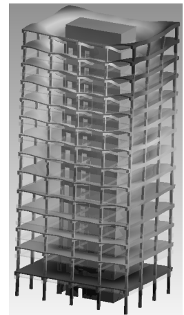
(f_{0(7)} = 8,7928 Hz) 7. Oscillation shape
