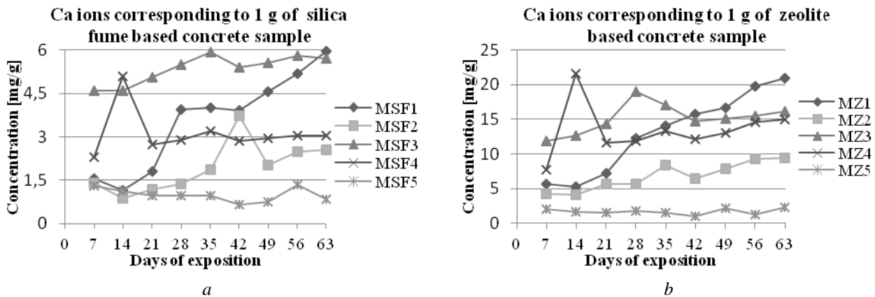
Fig. 2. Released ions of calcium corresponding to 1 g of concrete sample
